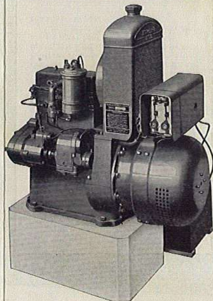
KOHLER Automatic Electric Plant
